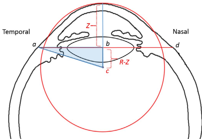
Figure 6. Mid-axial section of a schematic eye. The shaded triangle abc will be considered, where a is the temporal limbus, d is the nasal limbus, b is the midpoint of ad, and c is the center of the corneal “sphere.” In that triangle, ab = WTW / 2 , ac = R , the corneal radius, and bc = R - Z . Using Pythagoras theorem: R^2 = ab^2 + (R - Z)^2 , R - Z = \sqrt{R^2 - ab^2} , therefore Z = R - \sqrt{R^2 - \frac{WTW^2}{4}} .
