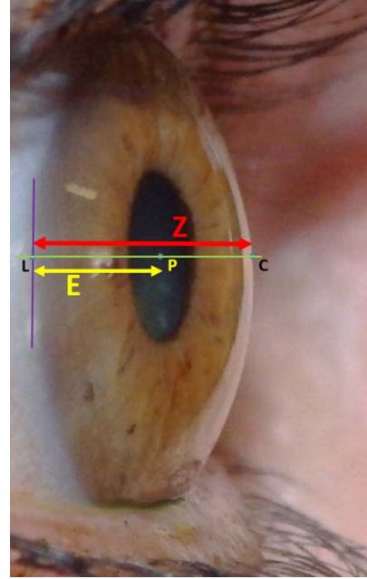
Figure 2. Lateral (temporal) perpendicular photograph of a right eye with a schematic outline of the photogrammetric method we used. The cross indicates the tangential limbus line (vertical, purple) and the limbus-pupil-cornea line (horizontal, green). The three blue dots mark the cardinal points, from left to right: Temporal limbal mark (L), mid pupil mark (P), and corneal mark (C). E, Lateral photographic temporal limbus to pupil distance; Z, Lateral photographic temporal limbus to cornea distance. The vACD is Z-E.
